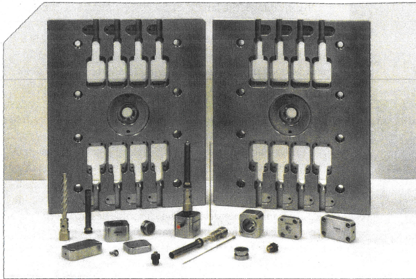
This array of mold parts, all produced in house, starts with a creative design and a wide range of materials.
