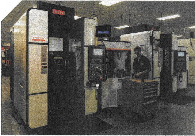
Yasda micromachining centers equipped with robotic part changers perform precision five-axis machining unattended in continuous operations through the weekend.
