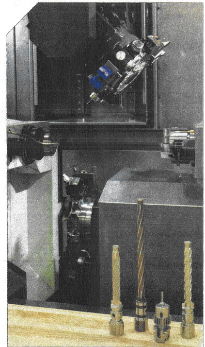
These examples show some of the variety of parts machined complete in one operation from barstock on three Nakamura-Tome multitasking machines that combine turning and milling operations in one machine.
