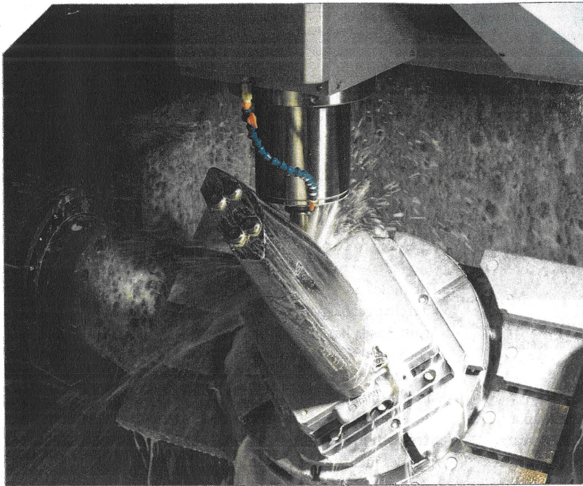
This 15-inch long core with its complex geometry is easy work for the Matsuura MX-850 which has big capacity and rigidity for heavy cutting with precision.
